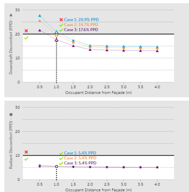
Figure 5 Thermal comfort conditions for three scenarios (blue, orange and purple curves for tall, punched and ribbon windows, respectively) with 40% window-to-wall ratio, double pane windows ( U=2 \text{ W/m}^2\text{K} ), outdoor temperature of -12^\circ\text{C} and indoor temperature of 23^\circ\text{C} . Tall windows generate too much downdraft to ensure a comfortable environment.
